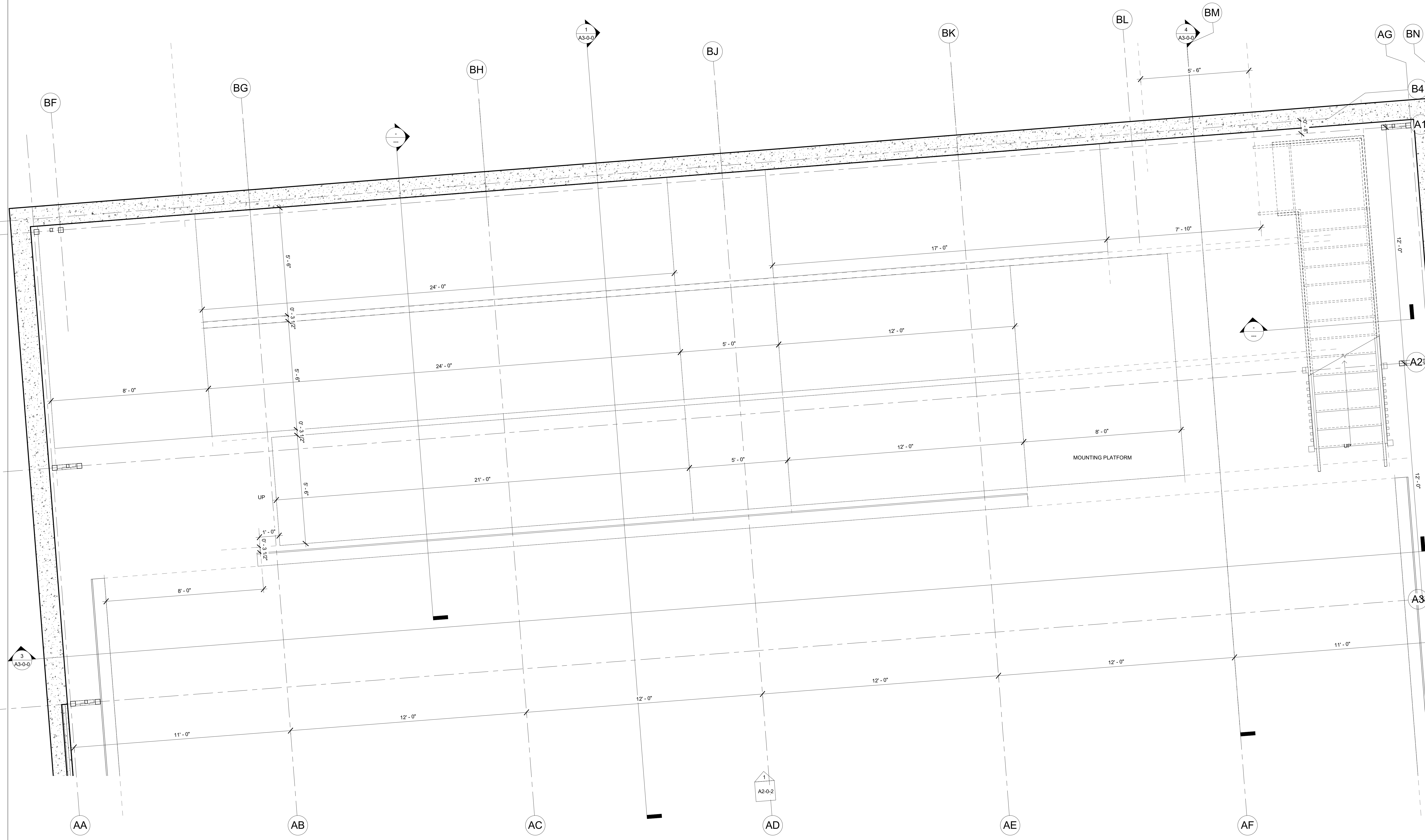
1 RAMP ENLARGED PLAN 1/2" = 1'-0"
